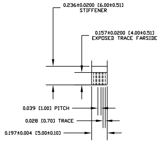
DETAIL A SCALE 2.0
